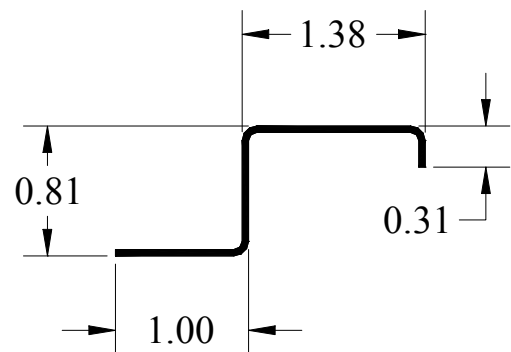
13/16" Z-Section
